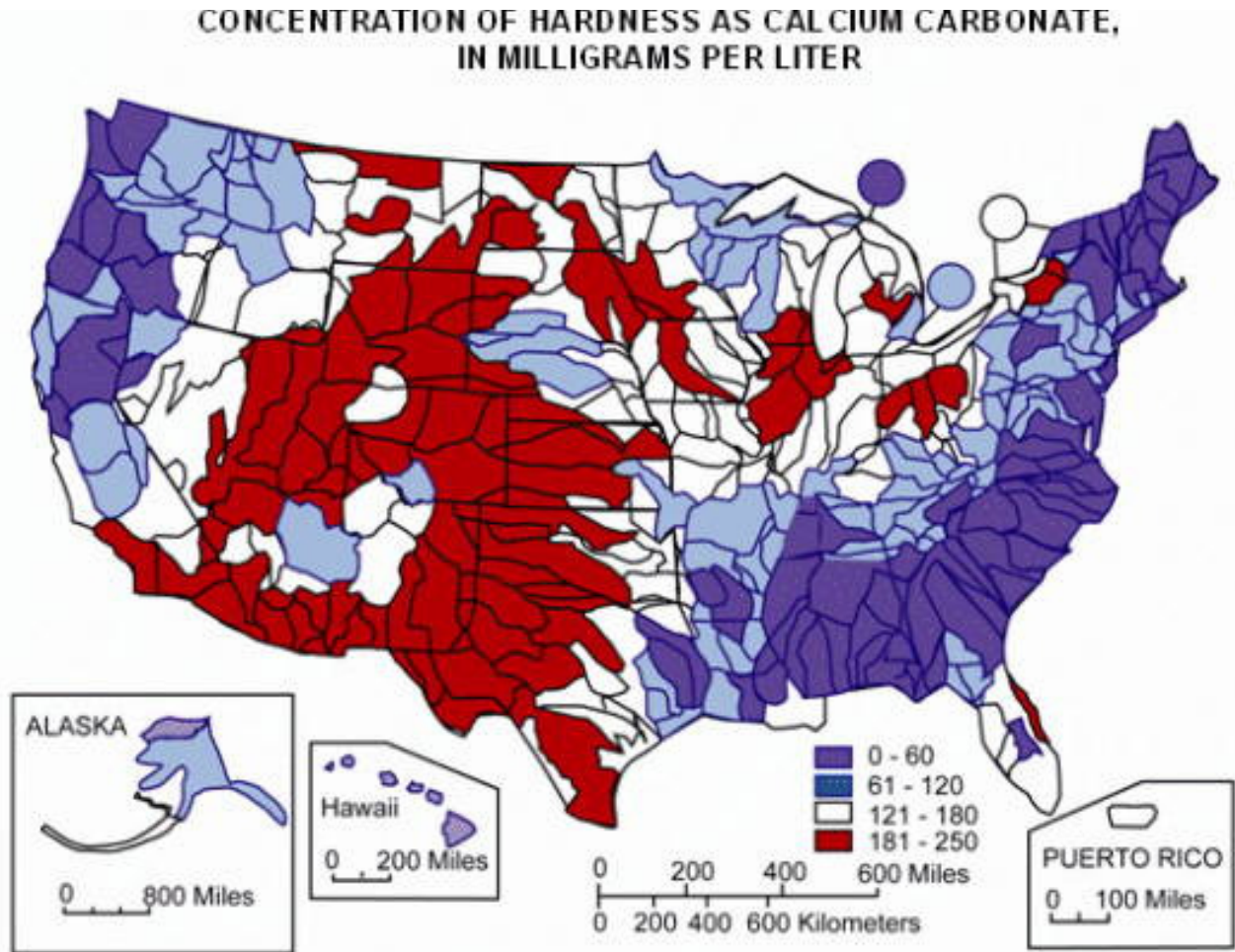
Mean hardness as calcium carbonate at NASQAN water-monitoring sites during 1975 water year. Colors represent site data representing streamflow from the hydrologic-unit rea. (Map edited by USEPA, 2005)
