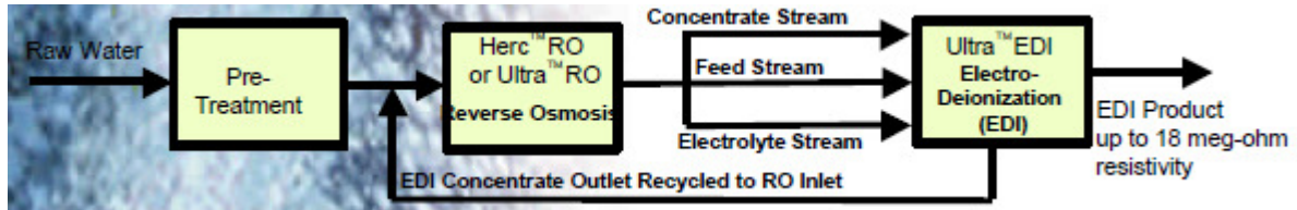
Typical Process Flow using Electro-Deionization (EDI) System
